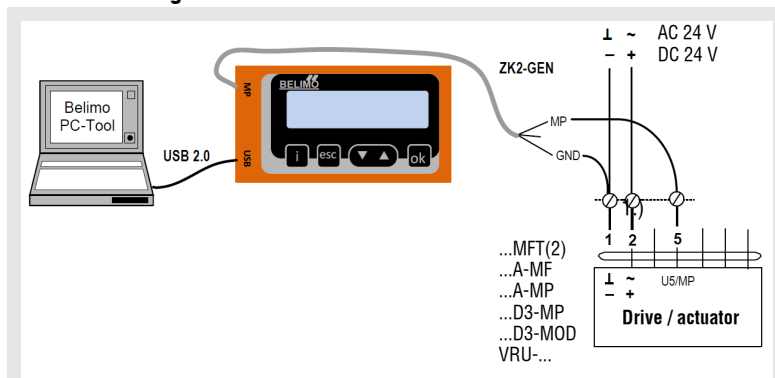
Connection diagram 2
