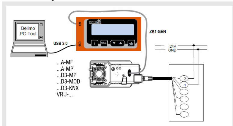
Connection diagram 1
