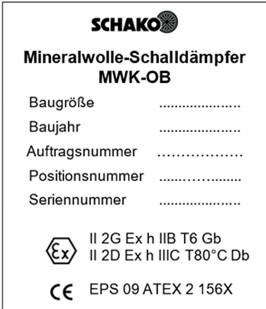
Figure 1: MWK-OB ATEX type plate
