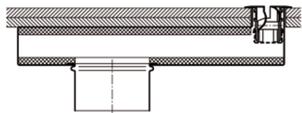
Floor slot diffuser model FBS-AUDIX
